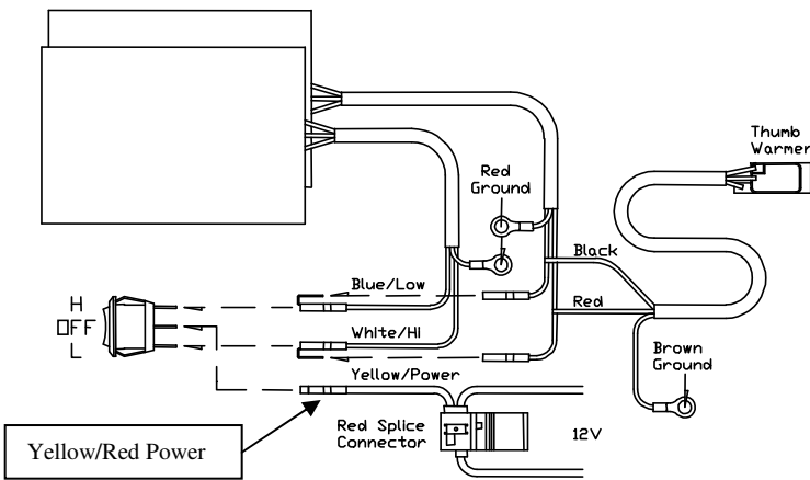
Figure 4. Hand Warmer w/Thumb Warmer Kits 210010 and 11
